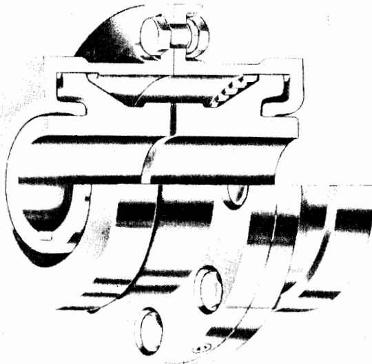
Fig. 4—All metal seal coupling.
