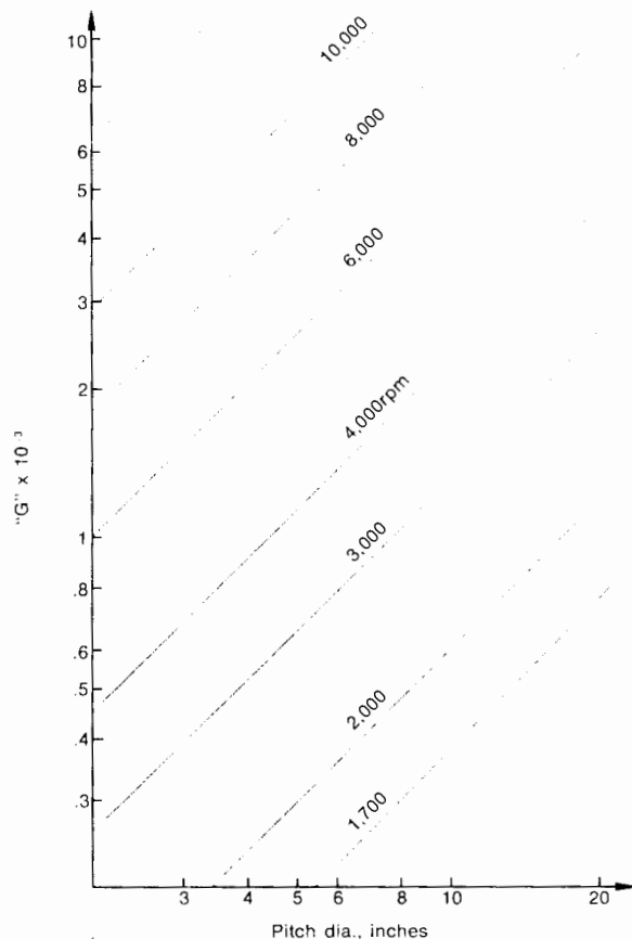
Fig. 2—Centrifugal forces in couplings.
